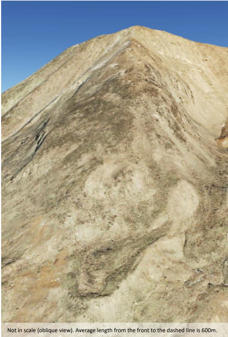
Creep of frozen ground
