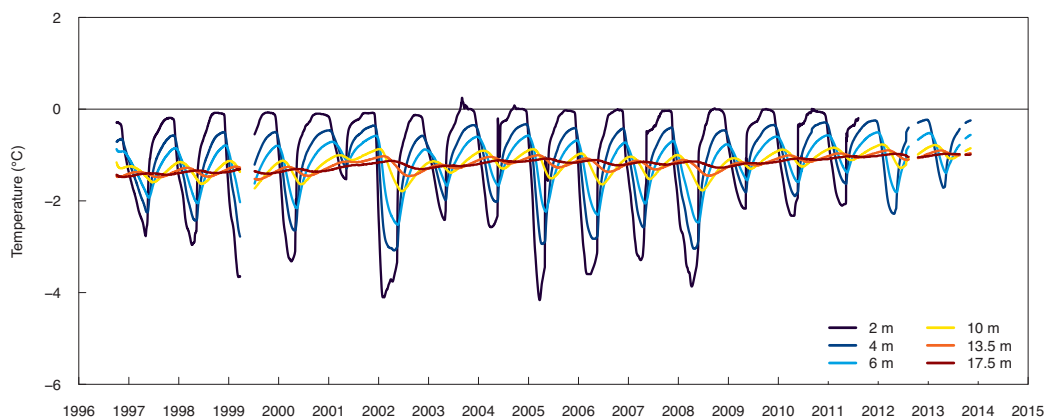
Figure A.15: Temperature-time series measured in the Muot Da Barba Peider 0296 borehole.
