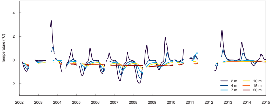
Figure A.23: Temperature-time series measured in the Schilthorn 5000 borehole.
