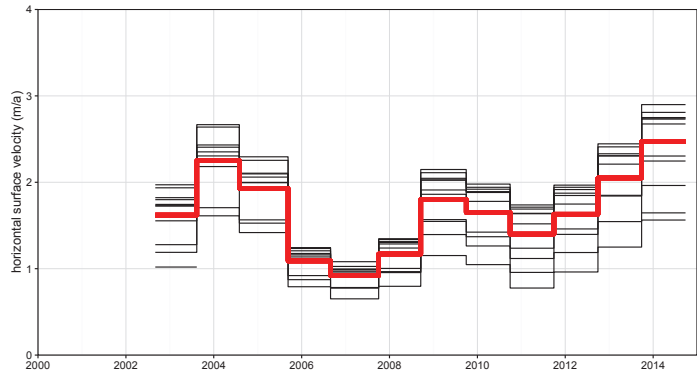
Figure A.33: Annual horizontal surface velocities at the Hungerlitälli3 kinematics site for individual points and the mean of the reference points (11, red line).
