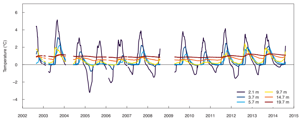
Figure A.16: Temperature-time series measured in the Muragl 0199 borehole.
