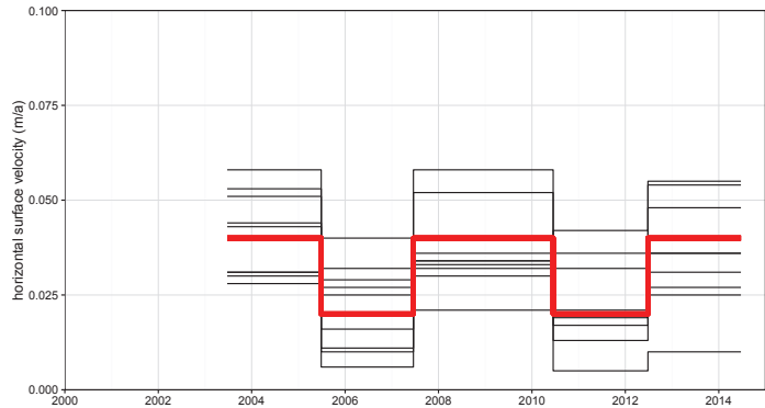
Figure A.29: Annual horizontal surface velocities at the Alpage de Mille kinematics site for individual points and the mean of the reference points (9, red line).
